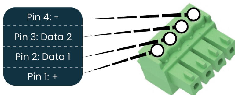
Figure 14: Expanded Mode Pixel Output Pinout
