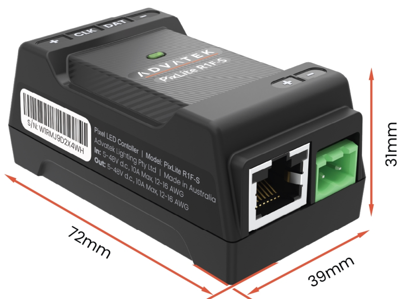
Figure 16: Receiver Mechanical Specifications
