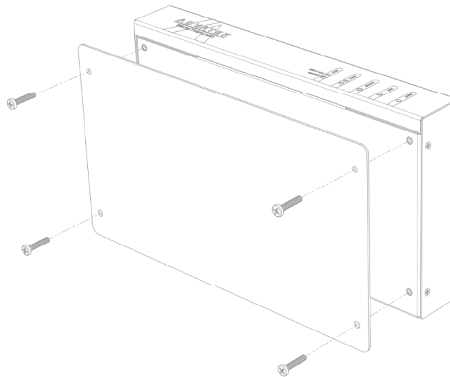
Figure 5: Controller Assembled onto Panel
