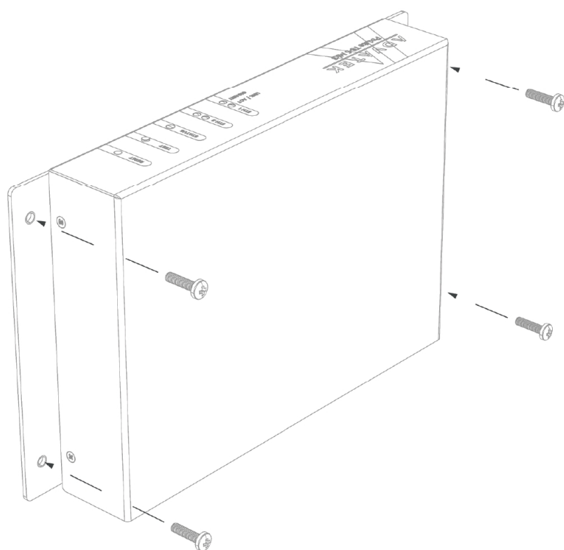
Figure 3: Mounting Plates Assembled to a Flat Surface
