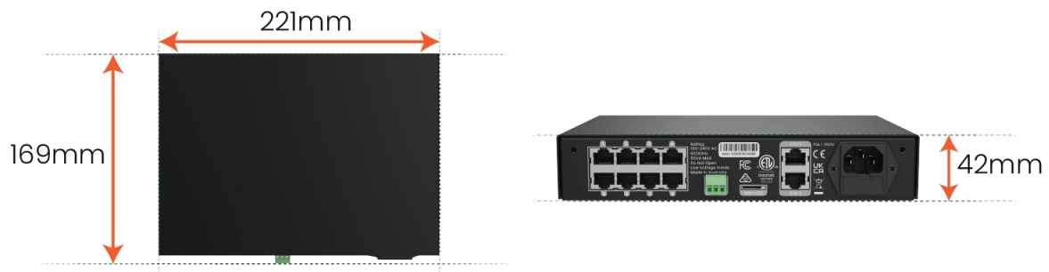
Figure 20: Mechanical Specifications
