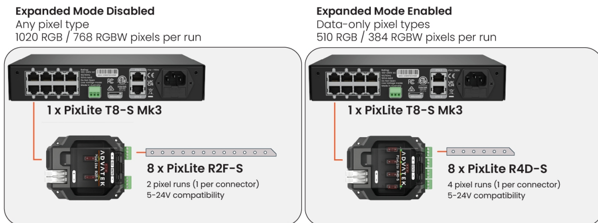
Figure 16: Connecting Receivers to Transmitter
